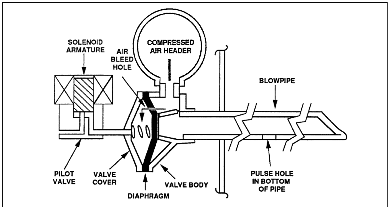
FIGURE 6-12. Normally closed solenoid valve
