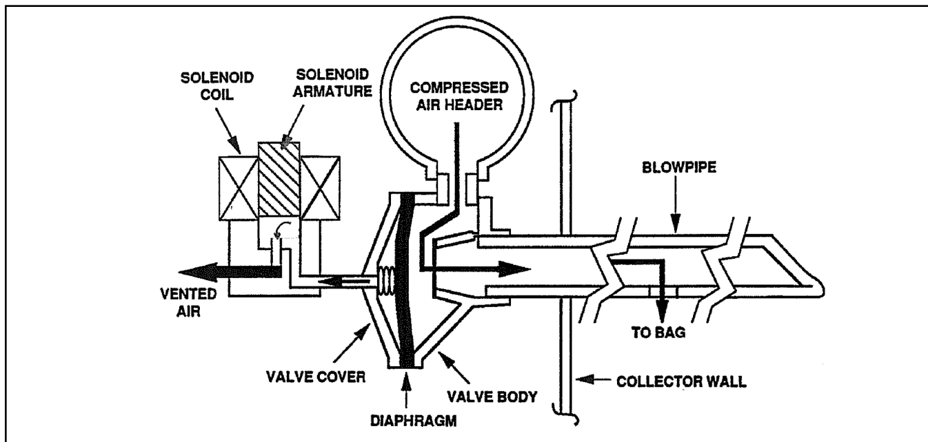
FIGURE 6-13. Solenoid valve – pulsing position
